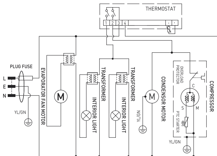
Circuit diagram (233924)
