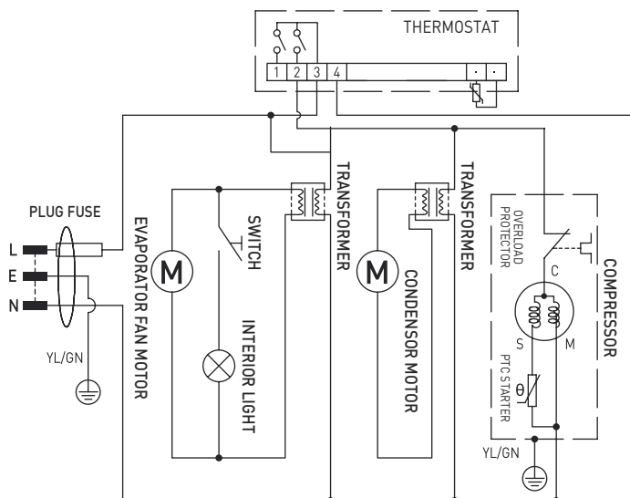
Circuit diagram (233924)
