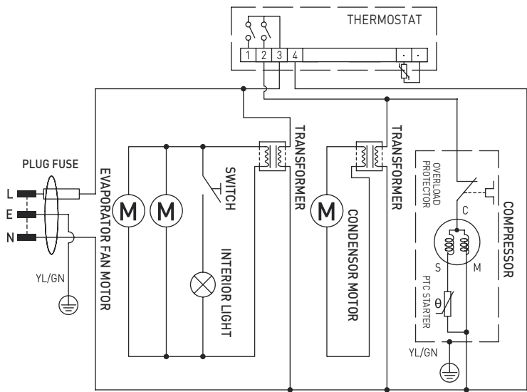
Circuit diagram (235836)
