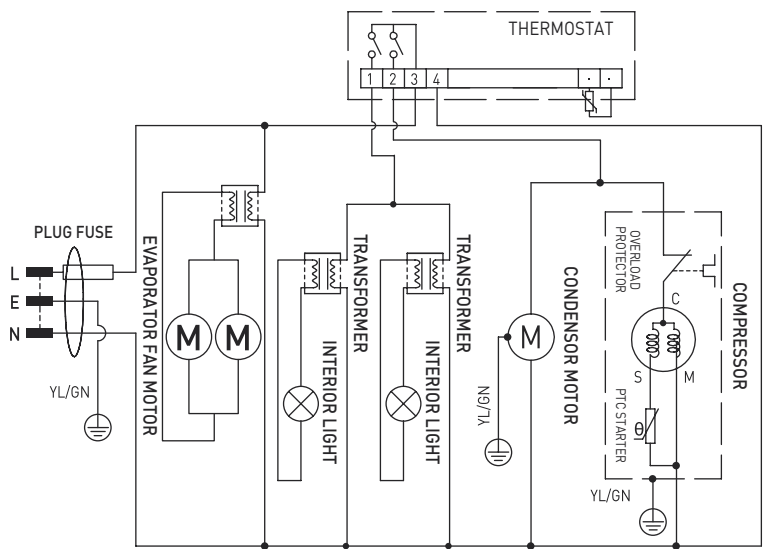
Circuit diagram (233931)
